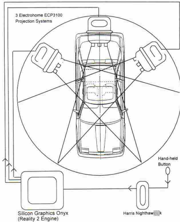
FIGURE 1 Top-down schematic of the University of Minnesota Human Factors Research Laboratory wrap-around simulation facility.
