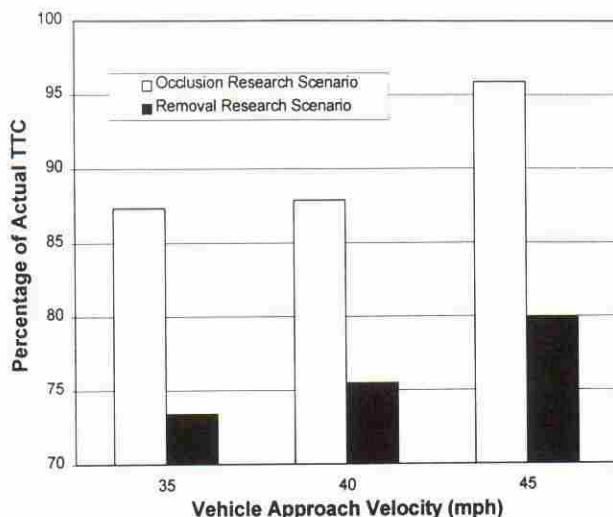
FIGURE 3 The main effect for research scenario and the main effect for vehicle approach velocity expressed as a function of each other. Estimated time-to-contact ( T_c ) scores have been converted to a percentage of T_c for comparative ease.
