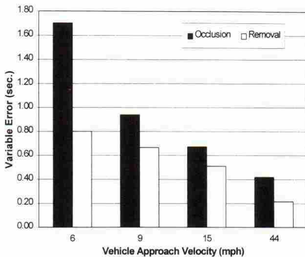
FIGURE 15 The interaction between vehicle approach velocity and research scenario for variable error. The interaction is a result of the dramatic decrease in variable error for the occlusion research scenario from the 6- to the 9-mph vehicle-approach-velocity condition as compared to the relatively mild decrease in variable error for the same vehicle approach velocities.
