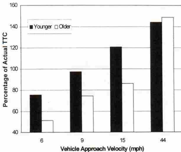
FIGURE 11 The Age \times Vehicle Approach Velocity interaction for the actual time-to-contact ( T_c ) analysis. Note, the actual T_c means have been converted to a percentage of actual T_c for ease of comparison.
