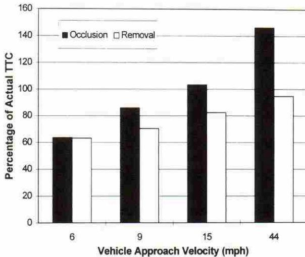
FIGURE 10 The Research Scenario \times Vehicle Approach Velocity interaction for the actual time-to-contact ( T_c ) analysis. Actual scores have been converted to a percentage of actual T_c to facilitate comparison.
